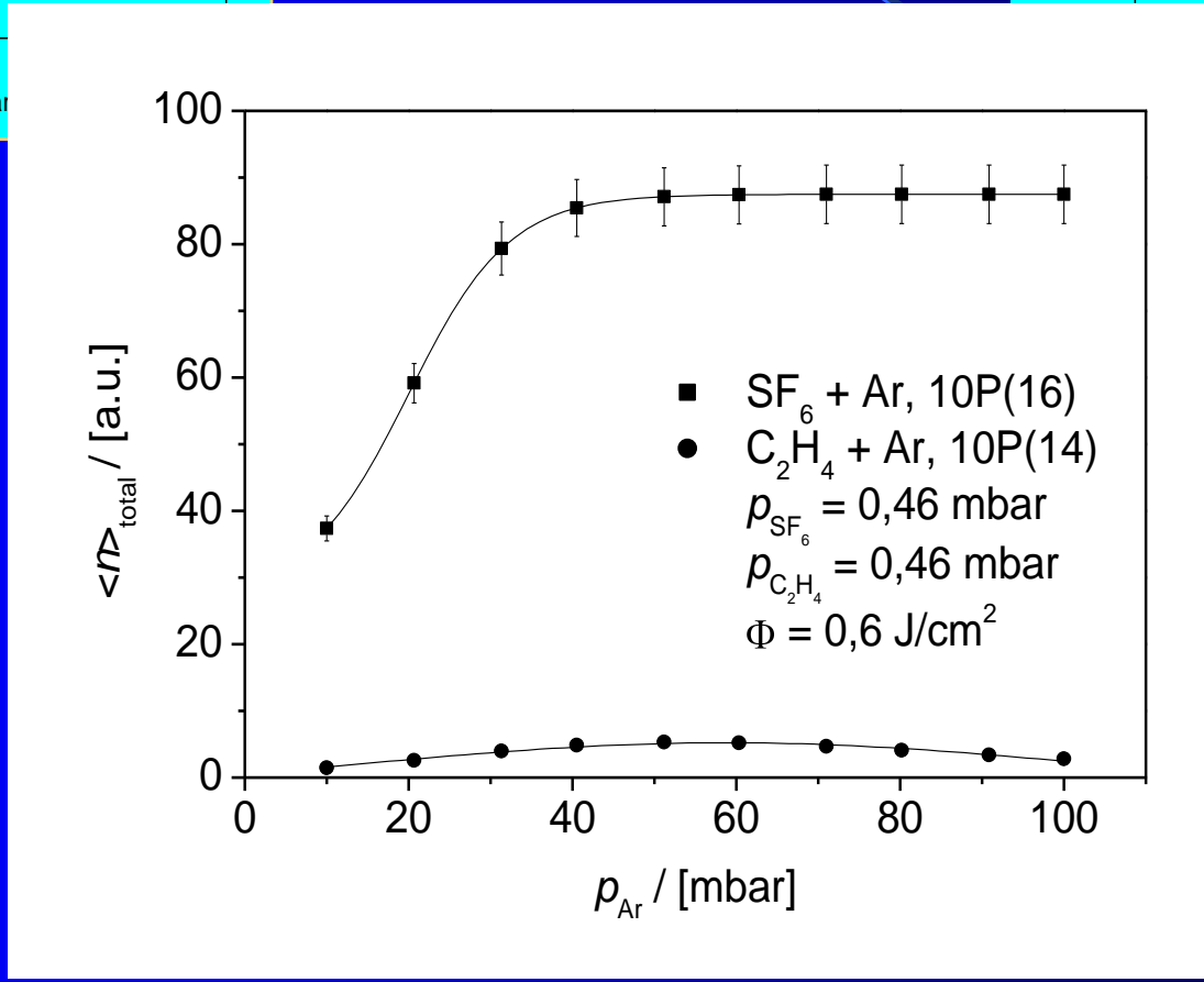
Comparison of total average number of absorbed photons \langle n \rangle_{\text{total}} for \text{SF}_6 and \text{C}_2\text{H}_4 molecule as a function of Ar buffer-gas pressure p_{\text{Ar}} , for \text{SF}_6 + \text{Ar} and \text{C}_2\text{H}_4 + \text{Ar} mixtures, under constant laser fluence F = 0,6 \text{ J/cm}^2 , at 10P(16) and 10P(14) line respectively.
